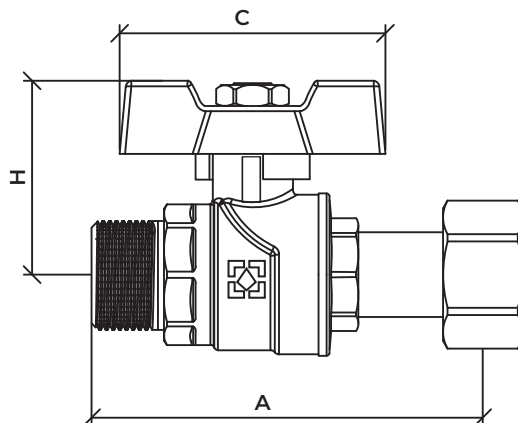
Ball valve straight with connectors series Black
