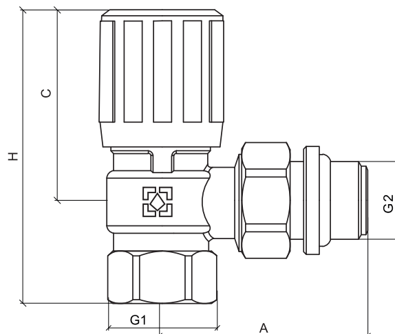
Angled manual adjustment valve MF
