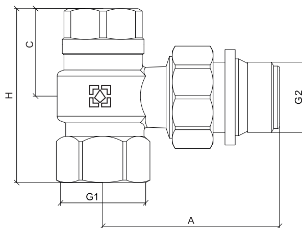
Adjusting angle valve MF
